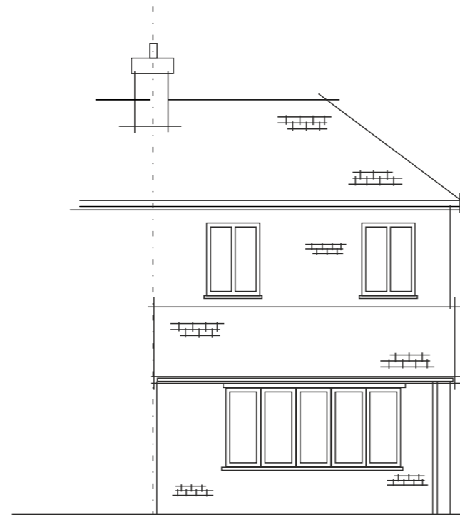
EXISTING FRONT ELEVATION (SOUTH)
