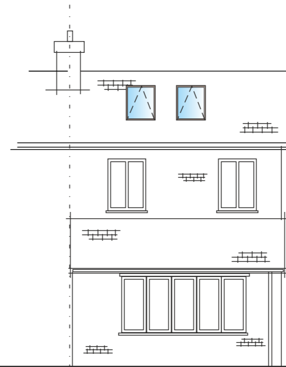
PROPOSED FRONT ELEVATION (SOUTH)
